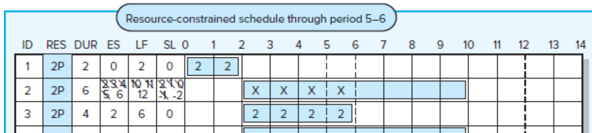
FIGURE 8.5 Resource-Constrained Schedule through Period 5–6
