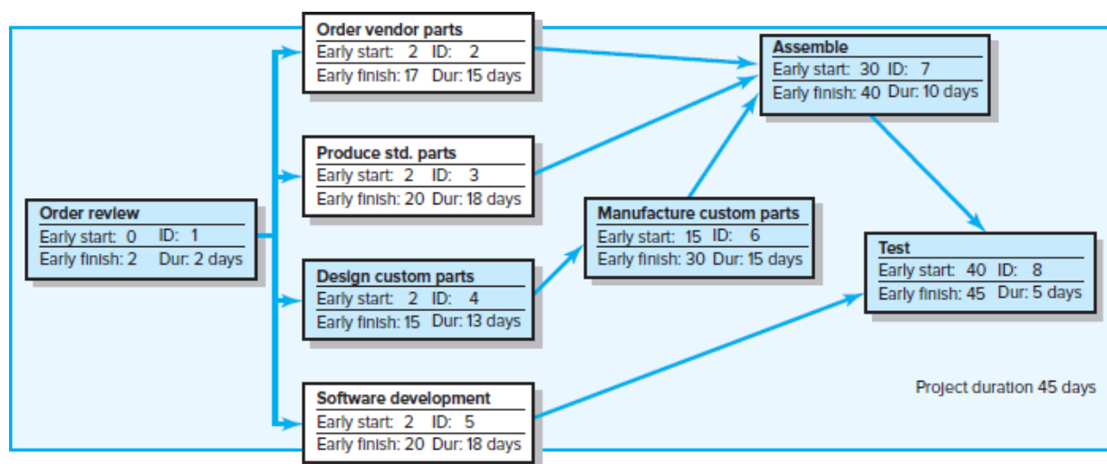
FIGURE A8.1A Air Control Project: Time Plan without Resources
